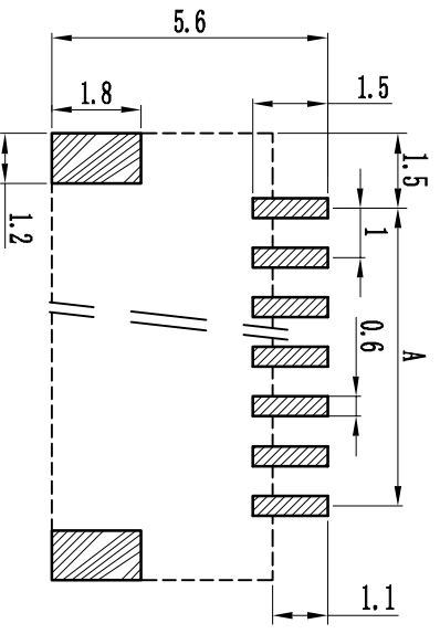
PCB Layout
