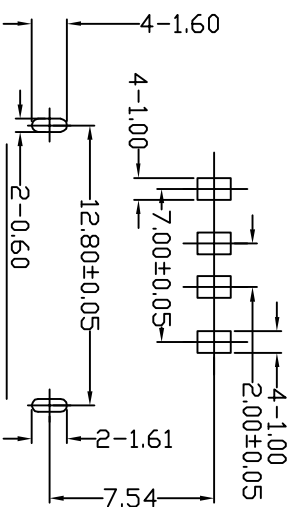
FRONT EDGE OF CONNECTOR PCB LAYOUT (T=1.60mm)
