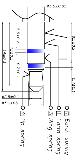
Matching Plug
